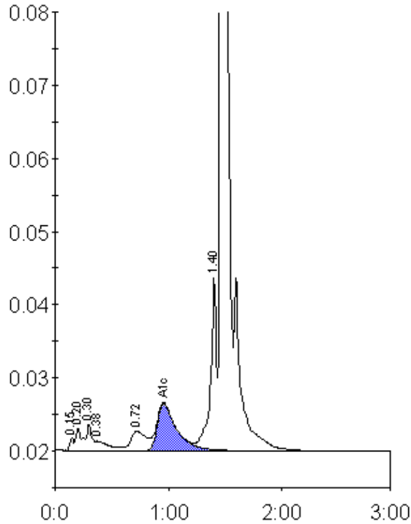
Peak table - ID: 10510092
